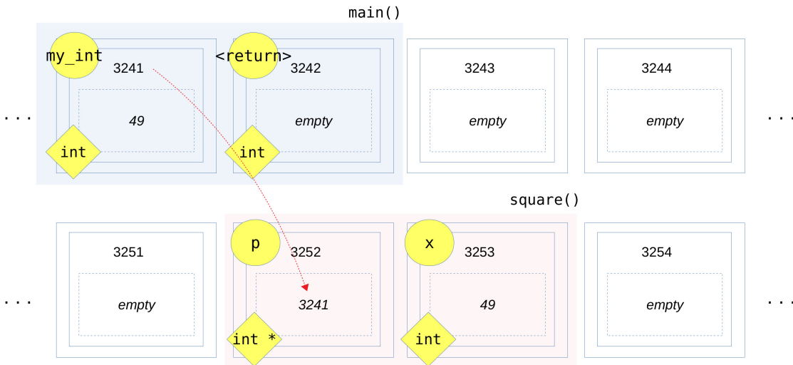
Figure 2.22: Memory model for the code in Example 2.7 after function square() has been processed, right before the memory reserved for square() is released .
