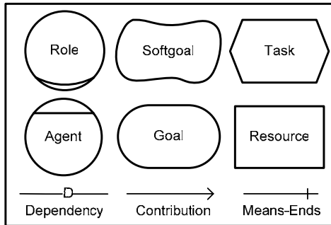
Figure 1 Selected elements of the i* framework
