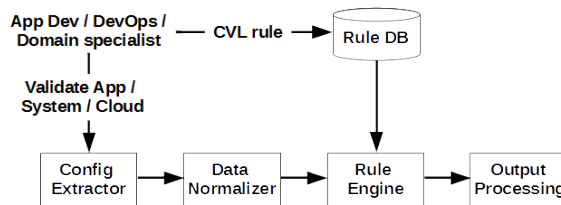
Figure 1. Conceptual Architecture of ConfigValidator . configuration storage and distribution systems like Akamai's ACMS [22].
