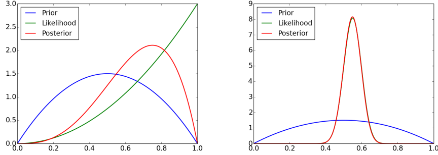
Figure 2: Plots of the prior, likelihood, and posterior for the coin flip example, with the prior Beta(2, 2). (Left) Small data setting, N_H = 2 , N_T = 0 . (Right) Large data setting, N_H = 55 , N_T = 45 . In this case, the data overwhelm the prior, so the posterior is determined by the likelihood. Note: for visualization purposes, the likelihood function is normalized to integrate to 1, since otherwise it would be too small to see.
