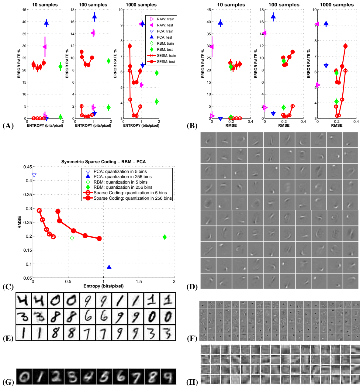
Figure 1: (A)-(B) Error rate on MNIST training (with 10, 100 and 1000 samples per class) and test set produced by a linear classifier trained on the codes produced by SESM, RBM, and PCA. The entropy and RMSE refers to a quantization into 256 bins. The comparison has been extended also to the same classifier trained on raw pixel data (showing the advantage of extracting features). The error bars refer to 1 std. dev. of the error rate for 10 random choices of training datasets (same splits for all methods). The parameter \alpha_s in eq. 8 takes values: 1, 0.5, 0.2, 0.1, 0.05. (C) Comparison between SESM, RBM, and PCA when quantizing the code into 5 and 256 bins. (D) Random selection from the 200 linear filters that were learned by SESM ( \alpha_s = 0.2 ). (E) Some pairs of original and reconstructed digit from the code produced by the encoder in SESM (feed-forward propagation through encoder and decoder). (F) Random selection of filters learned by RBM. (G) Back-projection in image space of the filters learned in the second stage of the hierarchical feature extractor. The second stage was trained on the non linearly transformed codes produced by the first stage machine. The back-projection has been performed by using a 1-of-10 code in the second stage machine, and propagating this through the second stage decoder and first stage decoder. The filters at the second stage discover the class-prototypes (manually ordered for visual convenience) even though no class label was ever used during training. (H) Feature extraction from 8x8 natural image patches: some filters that were learned.
