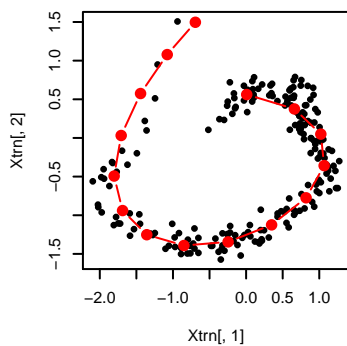
K: 15 s: 0.6 seed: 2 lpd: -1.49
