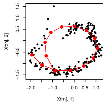
K: 15 s: 0.6 seed: 3 lpd: -1.583
