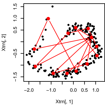
K: 15 s: 0.001 seed: 1 lpd: -1.49
