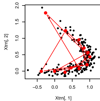
K: 15 s: 0.001 seed: 3 lpd: -0.302
