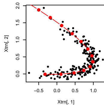
K: 15 s: 1 seed: 3 lpd: -0.266
