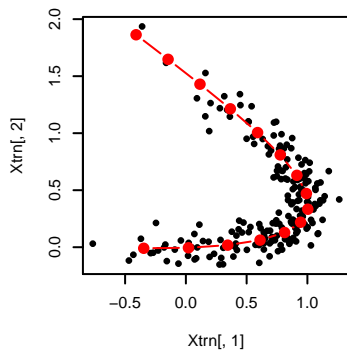
K: 15 s: 1 seed: 2 lpd: -0.261
