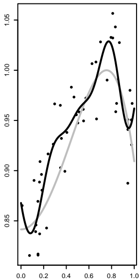
Gaussian basis function fit, s = 0.1 \lambda = 0.01
