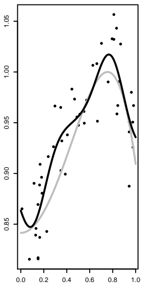
Bayesian fit, s = 0.1 \sigma = 0.031 \omega = 0.04
