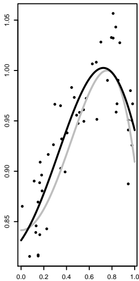
Gaussian basis function fit, s = 0.5 \lambda = 0.01
