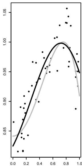
Bayesian fit, s = 0.5 \sigma = 0.033 \omega = 0.19
