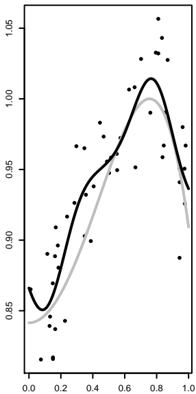
Gaussian basis function fit, s = 0.1 \lambda = 1
