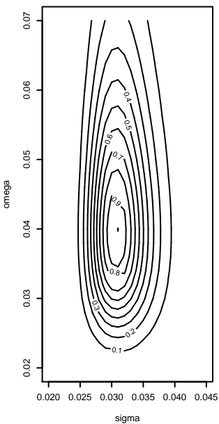
Bayesian fit, s = 0.1 \sigma = 0.031 \omega = 0.04
