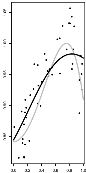
Gaussian basis function fit, s = 0.5 \lambda = 1
