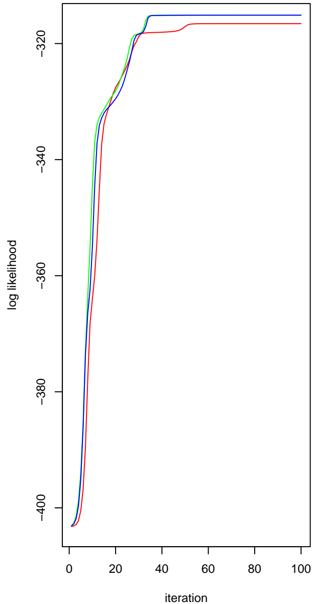
Three runs of EM for 5-component model
