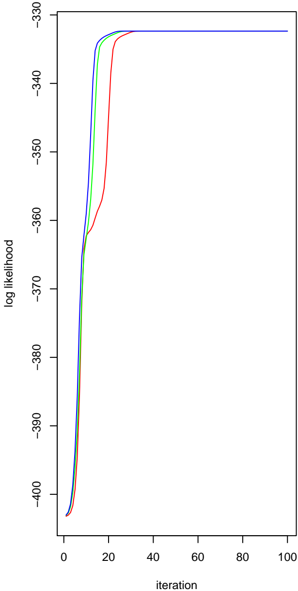
Three runs of EM for 3-component model
