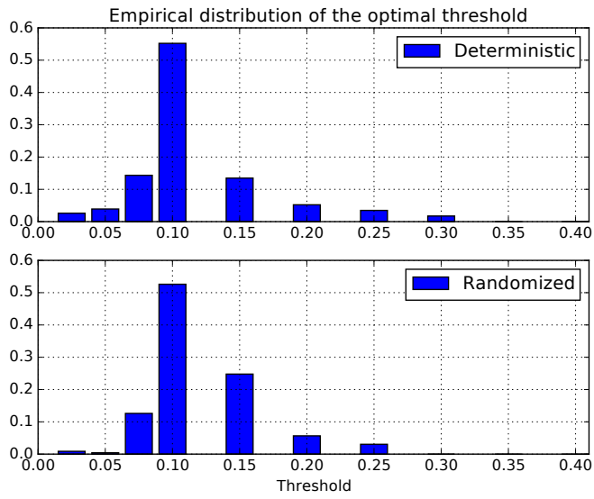
Fig. 6. Percentage of instances for which different threshold values are optimal.
