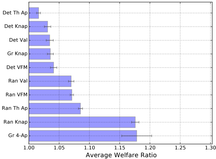
Fig. 3. Average welfare ratios for the Boston 2015 dataset containing 4-approval votes.
