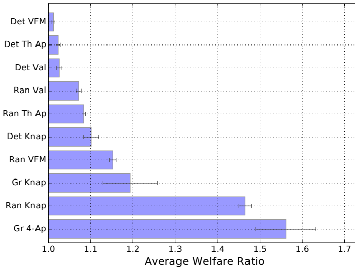
Fig. 4. Average welfare ratios for the Boston 2016 dataset containing knapsack votes.
