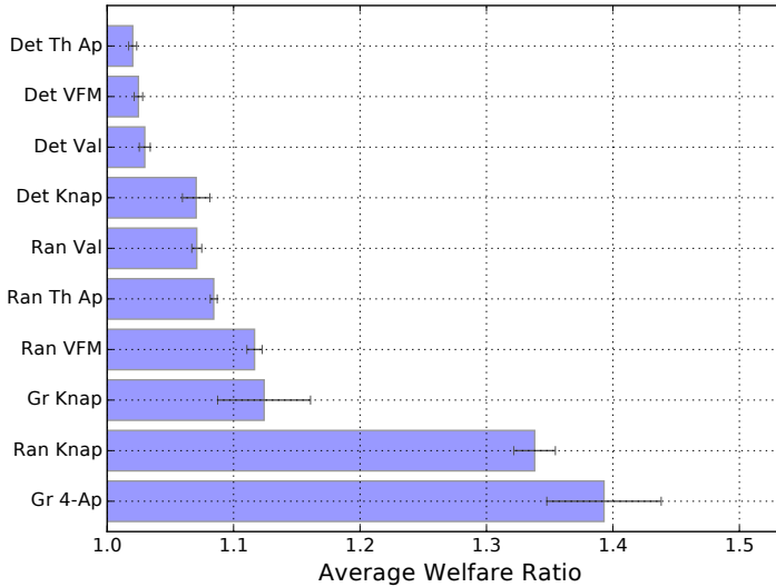
Fig. 1. Average welfare ratio (lower is better) of different approaches to participatory budgeting based on data from Boston 2015 and 2016 elections.
