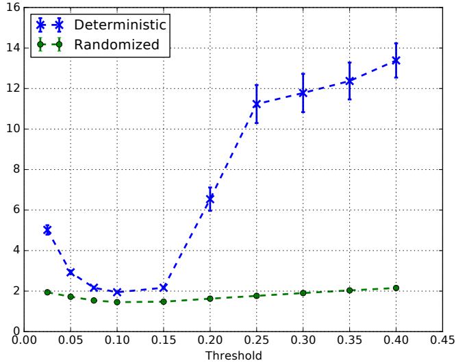
Fig. 5. Average distortion achieved by different threshold values in threshold approval votes.
