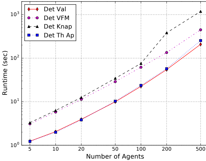
Fig. 2. Average running time of the deterministic voting rules on the Boston 2016 dataset.
