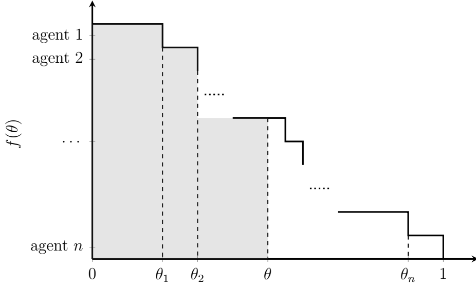
Figure 3: The illustrative picture of auxiliary function f(\theta) for a class i with n agents, sorted in ascending order of their values for the allocation. Each agent i corresponds to a rectangle defined by interval [0, \theta_i] on the x -axis, and interval [n - i, n - i + 1] on the y -axis. \int_0^\theta f(z) dz and \sum_{a \in N_i} \min(\theta, \sum_{o \in M} x_{a,o}) are two different ways to express the shaded area. The former integrates the height over interval [0, \theta] on the x -axis, while the latter sums the width over [0, n] on the y -axis.
