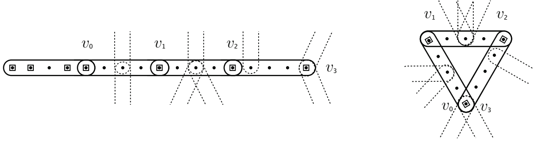
Figure 1: 2-linked paths with t = 3 . On the left v_0 \neq v_3 , while on the right v_0 = v_3 . Vertices in S are marked with a square.
