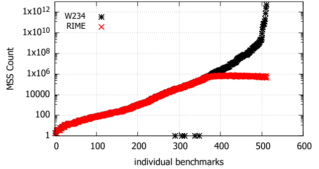
Figure 3: Scalability w.r.t. the MSS count.
