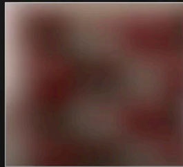
g_2(x, y)
