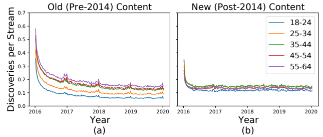
Figure 5: Expected rate of discoveries found from (a) older or (b) newer content as a fraction of all listening.
