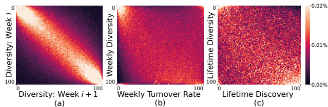
Figure 9: Distribution over diversity in adjacent weeks (a); diversity and turnover in the same week (b); diversity and discovery per stream across the entire trace (c). Variables are adjusted for activity and binned into percentiles.
