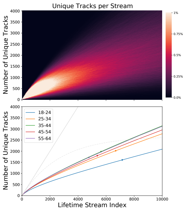
Figure 2: Top : distribution of users over the number of unique tracks listened, conditioned on stream count. Bottom : expected number of unique tracks per stream, per age group. Mean stream index after one year shown as dots. Identity (i.e., each stream is a discovery) shown in solid grey; draw-with-replacement curve shown in dashed grey.
