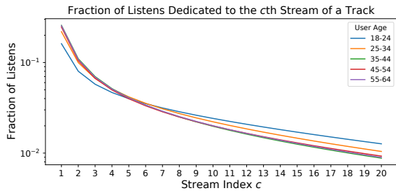
Figure 3: Number of times users listened to tracks for the c th time, normalized by total streams per user.
