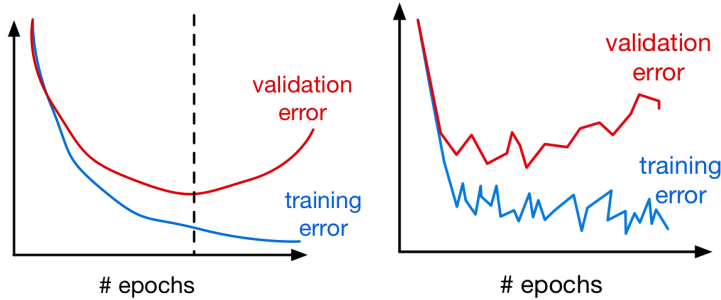
Figure 4: Training curves, showing the relationship between the number of training iterations and the training and test error. (left) Idealized version. (right) Accounting for fluctuations in the error, caused by stochasticity in the SGD updates.
