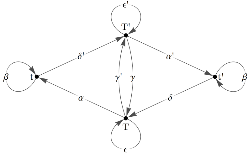
Figure 16: A directed graph, or finite automaton, for the generation of parent triangles from constituent triangles. Paths along the directed edges represent compositions of the mappings from Equations (1). Infinite paths along the directed edges may generate Penrose tilings of the plane.
