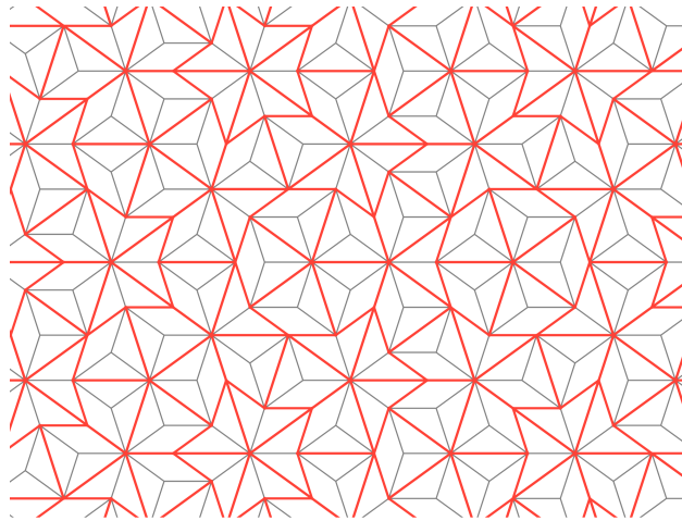
Figure 32: Kites and Darts tiling (red) mutually locally derived from Rhombs tiling (grey). Kites and Darts are derived according to local rules in Fig.31. Conversely, we see that Kites can derive one thin Rhomb, and halves of two thick Rhombs. While Darts also allow us to derive two halves of thick Rhombs. We see this since each Kite and Dart is composed of the same arrangements of Rhombs.
