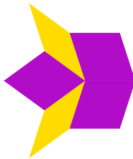
(c) As duals, this uniquely determines the Rhomb configuration
