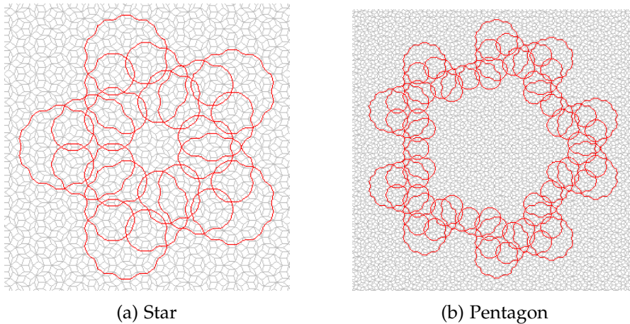
Figure 48: Two types of Flowers, figures by Stephen Collins [14].
