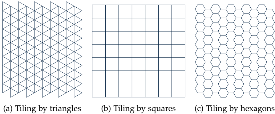
Figure 2: Regular tiling of the plane using single polygon protosets
