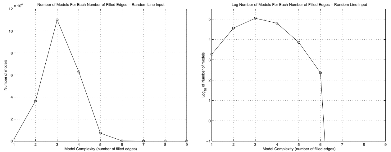
Figure 4.5: Same data as in 4.3, but collapsed along the epsilon odds axis.
