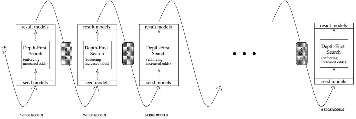
Figure 7.1: Schematic of Cascade Search – The search starts off looking for 1-edge models, starting from the empty model. It does so using no pruning criteria other than enforcing an increase in odds, as explained in Section 7.3. This produces a set of 1-edge result models. These result models are grouped and culled (G&C), as explained in Section 7.4, producing a smaller list of models which are then used as seeds/starting models for the next level of search. Note that at each stage, the depth-first search is looking for all k -edge models from all (k-1) -edge models. Several depth-first steps may be needed because collinear image segments can be added to existing model edges.
