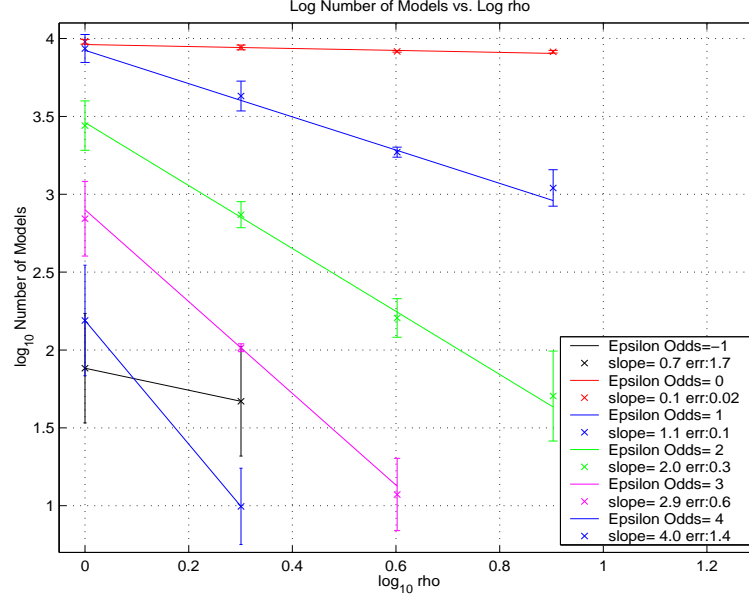
Figure 4.11: Results confirming the asymptotic behaviour of QP. Each line corresponds to the number of models found, at different resolutions, for a given epsilon odds. The slopes match the epsilon odds as predicted, except for epsilon odds of zero..
