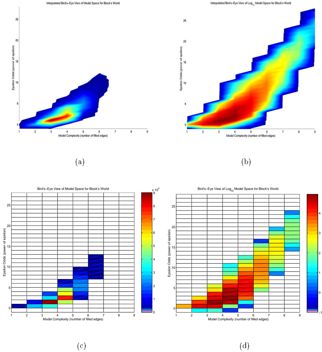
Figure 4.6: Number of models in \beta_{I_i} for aggregate data from six images from [20]. Data is broken down according to number of edges filled and epsilon odds. The top two images show interpolated versions, while the bottom two show the actual discrete data. The right most plots are \log_{10} versions. Their bins have been forced to a minimum of -1.
