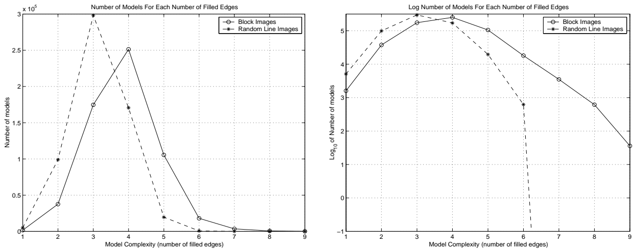
Figure 4.8: Same data as in Figures 4.6, but collapsed along the epsilon odds axis. Also shown for comparison is the data for random input images (Figure 4.5), which has been normalized so that the total number of models found is the same for both plots.
