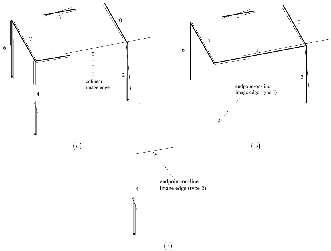
Figure 7.2: Examples of the only three types of image edges that can be added to a current model such that the increase in odds is sufficient. (a) image edge is collinear with model edge 1 (b) model edge 7 (and, incidentally, model edge 1) has endpoint on image line (c) image edge has endpoint on line formed by model edge 4 (and, incidentally, a type 1 endpoint on line with model edges 0 and 2)
