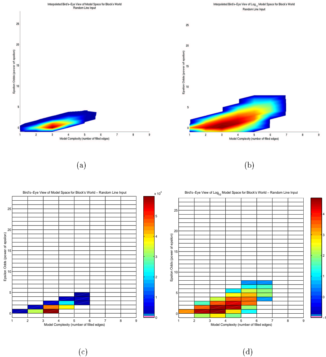
Figure 4.3: Number of models in \beta_{I_i} for aggregate data of ten random line images, broken down according to number of edges filled and epsilon odds. The top two images show interpolated versions, while the bottom two show the actual discrete data. The right most plots are \log_{10} versions. Their bins have been forced to a minimum of -1.
