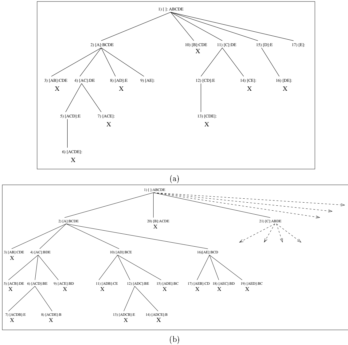
Figure 5.2: Alphabet World Depth-First Search for ACD and AE
