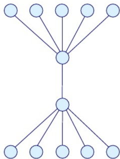
Input graph
