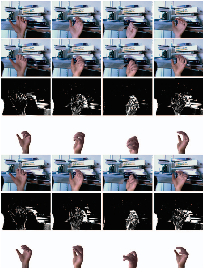
Fig. 10. Sequence 2: Each row shows, from top to bottom: (1) the observed image, (2) the final synthetic image with limited pose space, (3) the final residual image, (4) the synthetic side view with an angle of 45^\circ , (5) the final synthetic image with full pose space, (6) the residual image and (7) the synthetic side view.
