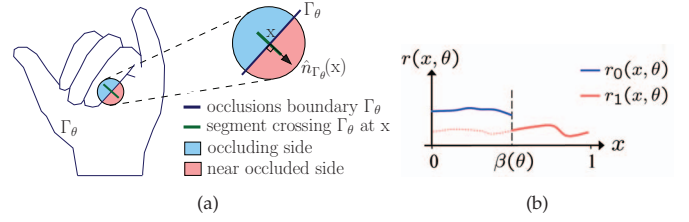
Fig. 5. (a) Example of a segment crossing the occlusions boundary \Gamma_{\theta} . (b) A curve representing the residual along this segment
