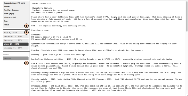
Figure 2: The baseline system, featuring (1) patient information panel, (2) a list of clinical notes, and (3) a search bar.
