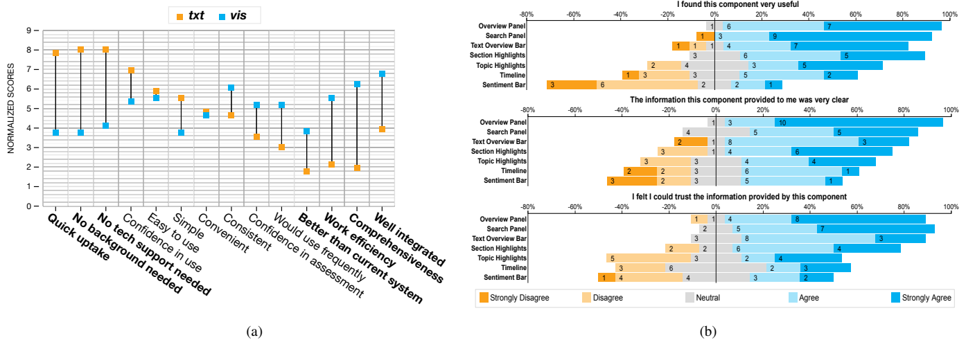
Figure 3: (a) Normalized scores (higher is better) for the adapted System Usability Scale for the baseline condition ( txt ) and MedStory ( vis ) ( bolded items: p < .05 ); and (b) Likert assessment of MedStory components.
