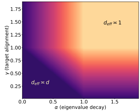
Figure 1: d_{\text{eff}} according to Corollary 6.
