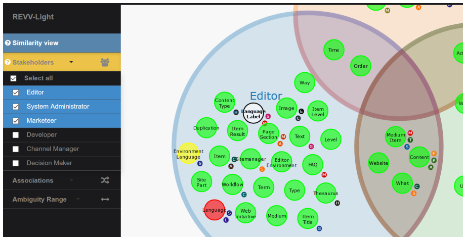
Figure 5: The REVV-Light tool showing an excerpt of the CMS-Company data set.
