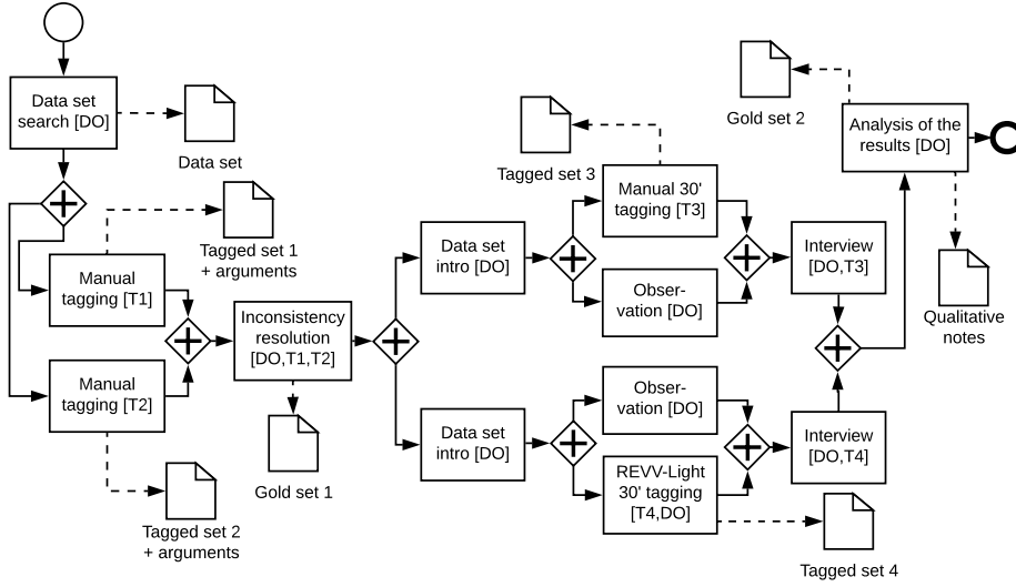
Figure 6: BPMN diagram of the experimental protocol for one data set. The following labels denote the roles the student groups play: DO is the data owner, i.e., the group who retrieved the user stories; T1 and T2 are the groups who independently tagged the data set without time constraints; T3 is the group that did the manual, time-constrained tagging; T4 is the group that did the time-constrained tagging with REVV-Light. For readability, only output data flows are shown.
