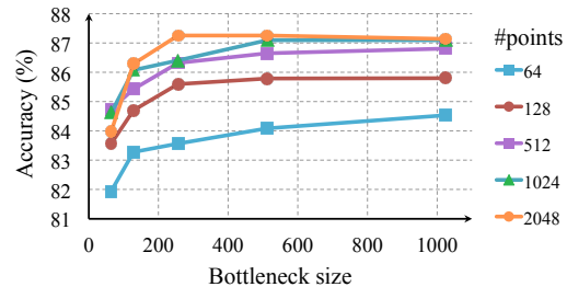
Figure 15. Effects of bottleneck size and number of input points. The metric is overall classification accuracy on ModelNet40 test set.
