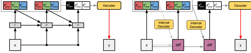
Figure 8: AIR vs. DAIR : Left : The standard AIR architecture. Right : The DAIR architecture. At each time-step i , the latent variables produced so far are used to perform a partial rendering of the scene. The difference of this partial rendering from the image under question is used infer z_{\text{pres}}^i , z_{\text{what}}^i and z_{\text{where}}^i in the current time-step.
