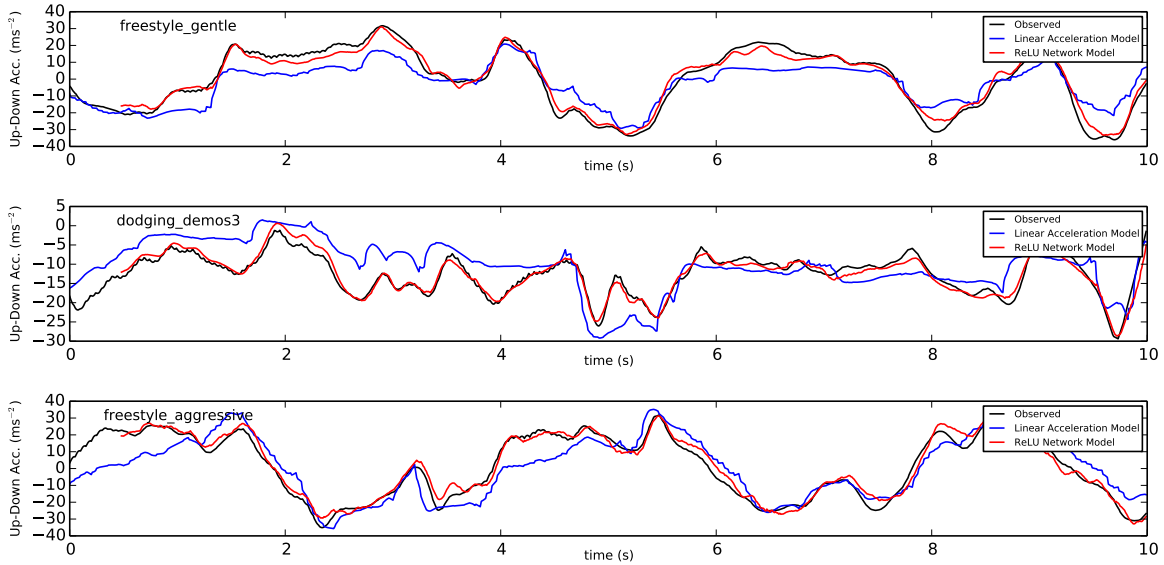
Figure 4: Observed and predicted accelerations in the up-down direction over three difficult test-set trajectories corresponding to different aerobatic maneuvers. In all cases, the baseline Linear Acceleration Model captures the gross pattern of the acceleration over the maneuver, but performs very poorly compared to the novel ReLU Network Model.
