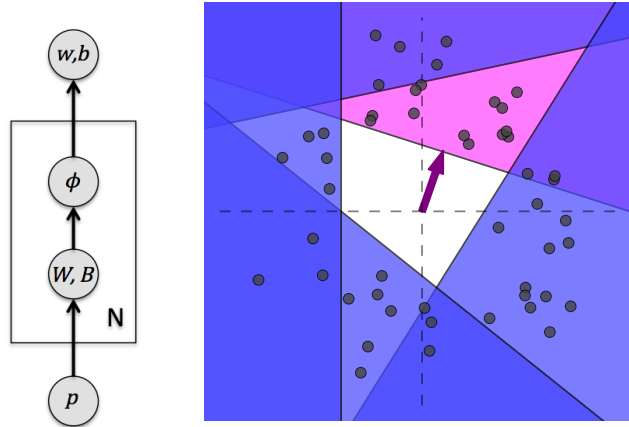
Figure 2: Left: A diagrammatic representation of the neural network used in the ReLU Network Model. Input p is sent to each of N hidden units. Each unit computes the inner product of p and W_i , the weight vector for that unit. A bias B_i is added, and the result sent to the unit activation function, \phi(\cdot) = \max(\cdot, 0) . This rectified-linear activation function simply zeroes its input if negative. The outputs of all hidden units are then linearly mixed by the output unit, with weights w and bias b . Right: A pictorial representation of the flexibility of the ReLU Network Model. Each hidden unit can be thought of as defining a hyperplane (line) in the 2D input space pictured. The data points (grey) each fall somewhere in input space and each has a value we wish to regress (not pictured). Consider the hidden unit i , drawn in purple. The purple arrow points in the direction of weight vector W_i , and has length according to B_i . Points on one side of this line do not activate unit i , while points on the other side (shaded) cause positive output. This effectively partitions the input space, and the partitions generated by considering many hidden units (blue) together split the space into regions. These regions give the model flexibility to capture structure in the input data. In the ReLU Network Model, the partitions are learned from data.
