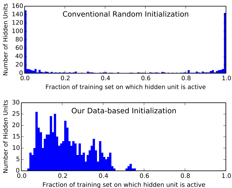
Figure 5: Histograms of hidden unit activation over the training set, showing the advantage of our data-based initialization method. Hidden units which fall at either end of the histogram, being either always active or always inactive, are not useful to the ReLU Network Model. Our initialization method does not produce any units which are not useful, and requires no tuning or setting of hyperparameters.
