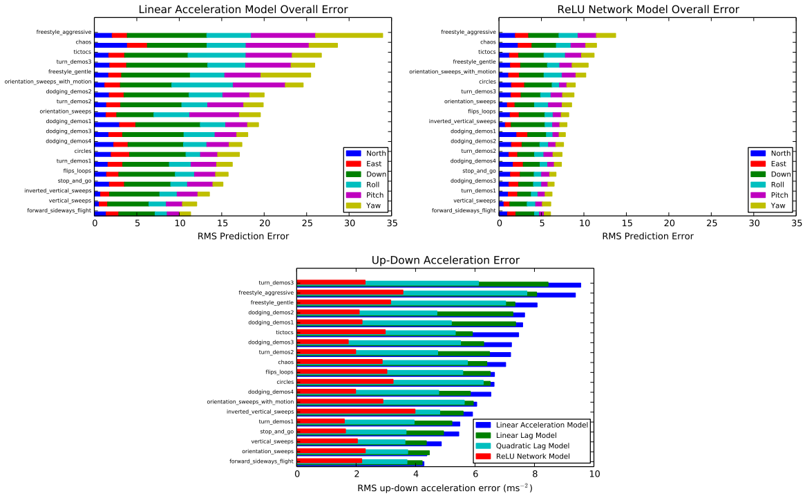
Figure 3: Performance Comparison of the ReLU Network Model and baseline models from Section 3. Top Left: Overall RMS prediction error of the Linear Acceleration Model over all acceleration components, each denoted by a different color. Top Right: Overall RMS prediction error of the ReLU Model over all acceleration components. Across all maneuvers, this result represents a 58% improvement in RMS error over the Linear Acceleration Model above. Bottom: RMS Error in predicting the up-down acceleration of the helicopter on test-set trajectories, which is empirically found to be the most difficult component to predict. The Linear Acceleration Model (blue) is outperformed successively by the Linear Lag Model which accounts for control lag, and the Quadratic Lag Model which accounts for some simple nonlinearities. The ReLU Network Model significantly outperforms all baselines, demonstrating the importance of accounting for hidden system state. Performance is displayed separately for each maneuver, but the labels are not used during training. Across all maneuvers, the ReLU Network Model reduces up-down RMS error of the Linear Acceleration Model by 60% .
