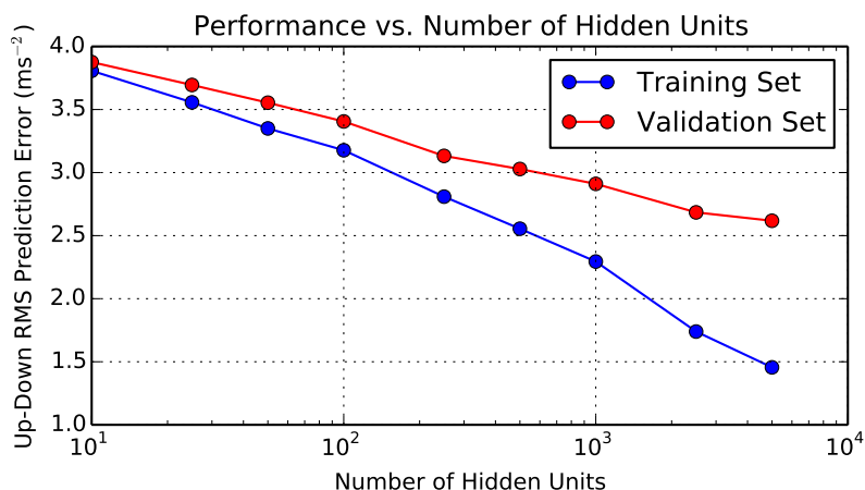
Figure 6: Training and validation set performance as a function of the number of hidden units ( N ) used in the ReLU Network Model. Training time increases linearly with N . Training set performance decreases as more units are added, but validation set performance levels out indicating that further model complexity is not required. In our performance experiments we use N = 2500 hidden units.
