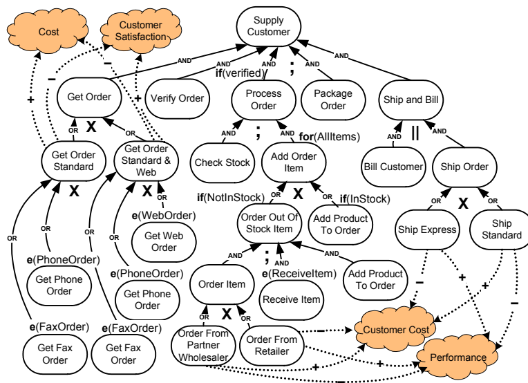
Fig. 2. A goal model for the “Supply Customer” business process
