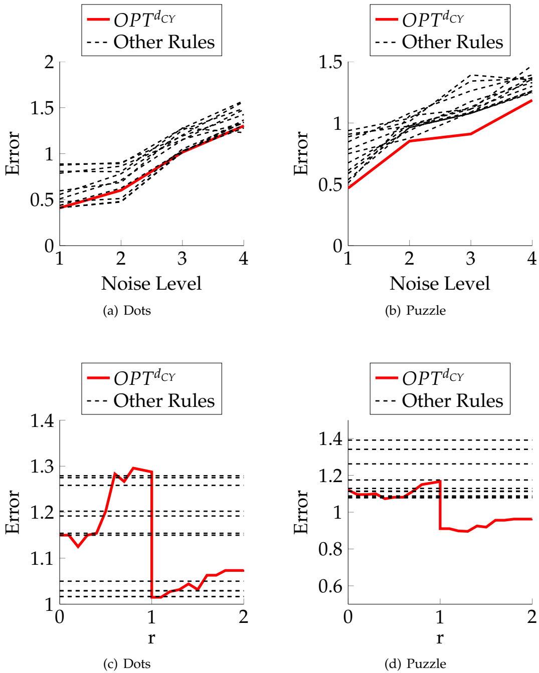
Figure D.2: Results for the Cayley distance ( d_{CY} ): Figures D.2(a) and D.2(b) show that OPT^{d_{CY}} outperforms other rules given the true parameter, and Figures D.2(c) and D.2(d) (for a representative noise level 3) show that it also outperforms the other rules with a reasonable estimate.
