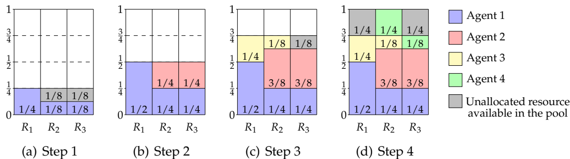
Figure 5.1: Allocations returned by DYNAMIC DICTATORSHIP when agent 1 reports its true demand vector.
