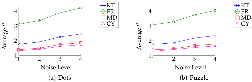
Figure 9.1: Positive correlation of t^* with the noise parameter
