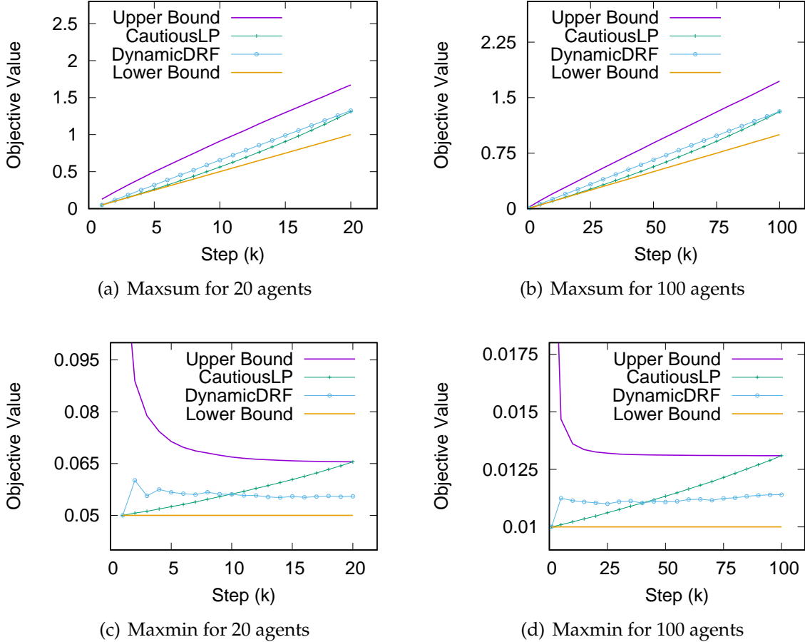
Figure 5.4: The maxsum and maxmin objectives as a function of the time step k , for n = 20 and n = 100 .
