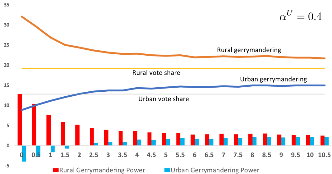
Figure 4: The number of districts won (top) and gerrymandering power (bottom) compared to \phi for \alpha^U = 0.4 .
