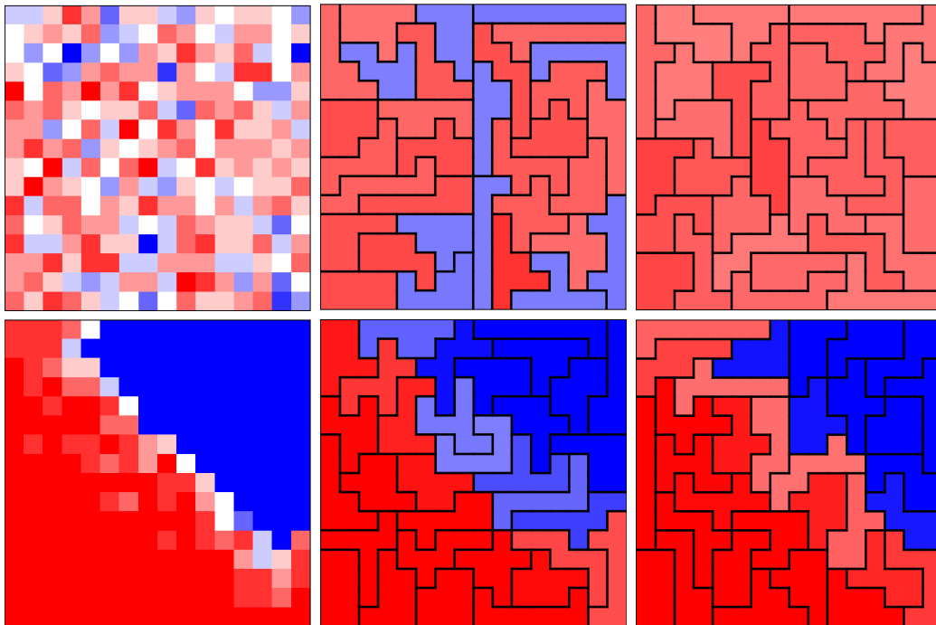
Figure 2: An example of the gerrymandered solutions B^+ found when \alpha^U = 0.4 . Top row \phi = 0 bottom row \phi = 10 . First column is partisan distribution of voters (similar to Figure 1). Second column is the gerrymandered solution for U , third column is the gerrymandered solution for R . Colour intensity within a district increases with the strength of victory.
