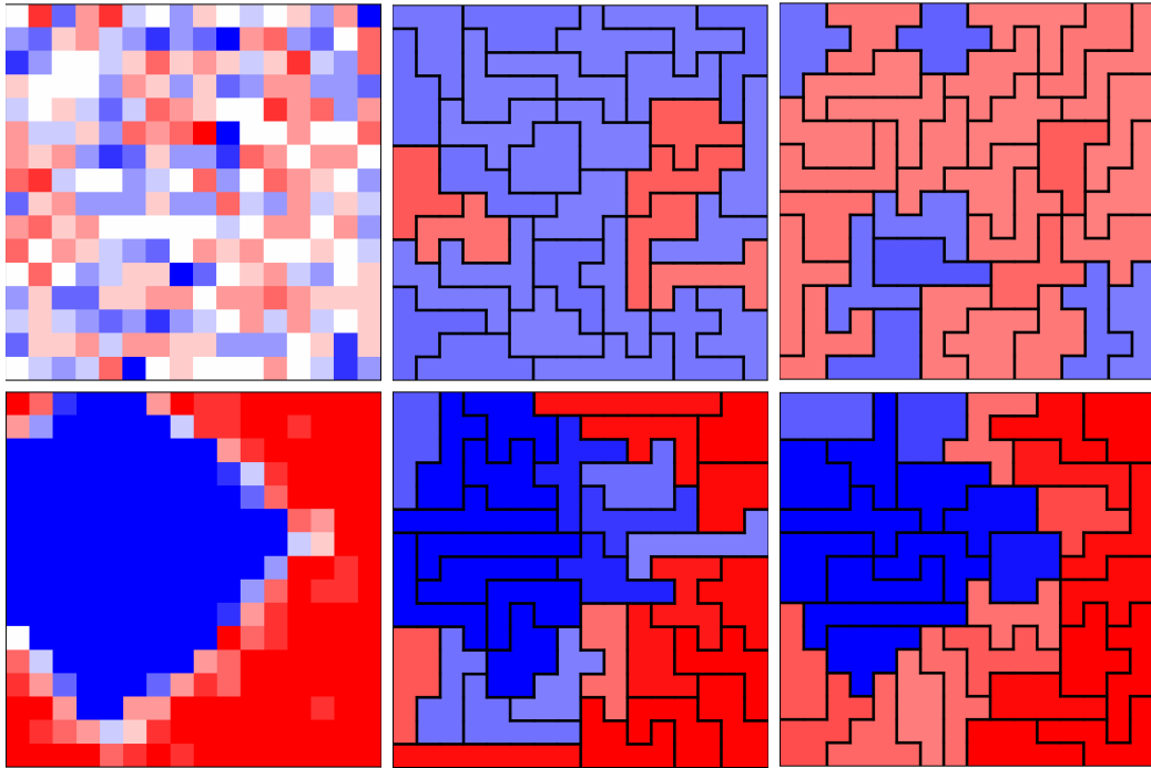
Figure 5: An example of the gerrymandered solutions B^+ found when \alpha^U = 0.5 . Top row \phi = 0 bottom row \phi = 10 . First column is partisan distribution of voters (similar to Figure 1). Second column is the gerrymandered solution for U , third column is the gerrymandered solution for R . Colour intensity within a district increases with the strength of victory.
