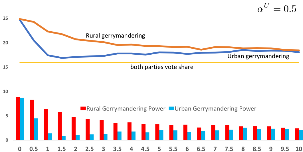
Figure 6: The number of districts won (top) and gerrymandering power (bottom) compared to \phi for \alpha^U = 0.5 .
