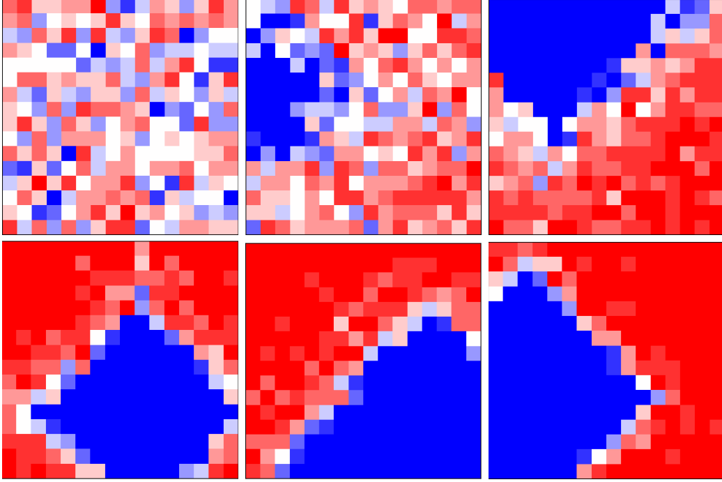
Figure 1: Partisanship distribution for \alpha^U = 0.45 and various values of \phi ( \phi = 0, 1, 3 in the top row from left to right and \phi = 5, 7, 9 in the bottom row from left to right). Blue/red represents a majority of U/R voters, and colour intensity increases with the majority strength.
