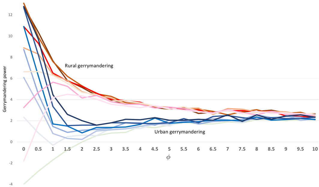
Figure 3: The average gerrymandering power of the parties versus \phi . The urban/rural party is in blue/red, and a darker colour represents a higher vote share of the gerrymandering party.
