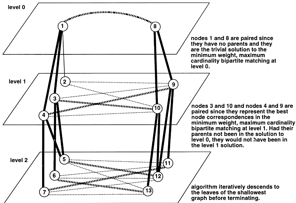
Fig. 9. Illustration of the SMGBM algorithm (see text for explanation).
