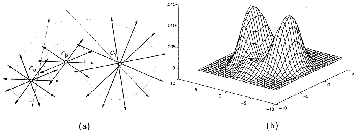
Fig. 3. (a) The clusters formed by the centers of the 1D SSCs, associated with the cross-sections through an object. (b) One of the filter kernels \delta(\Theta, x, y) used in computing the saliency of the SSCs Eq. (3). The kernel is obtained by computing the oriented energy at \Theta = 0^\circ for a disc.
