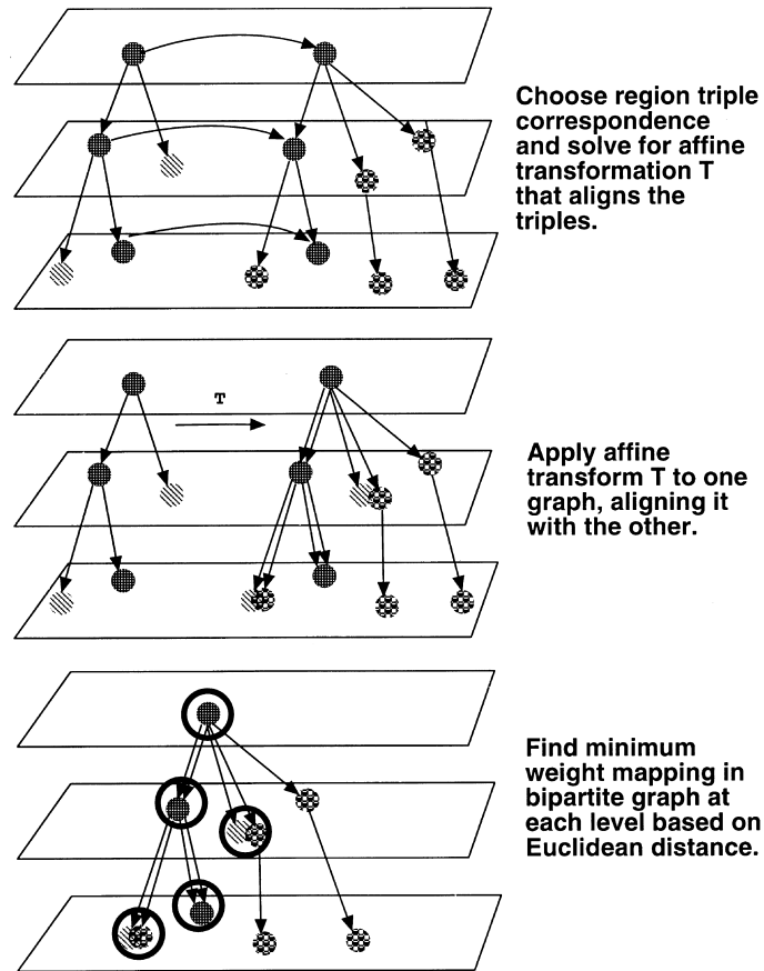
Fig. 10. Illustration of the SMGAT algorithm (see text for explanation).
