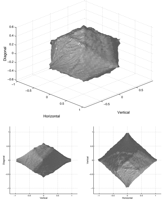
Figure 10: An equi-surface of 3d joint histogram of horizontal component, its vertical cousin and diagonal cousin, viewed from three different angles
