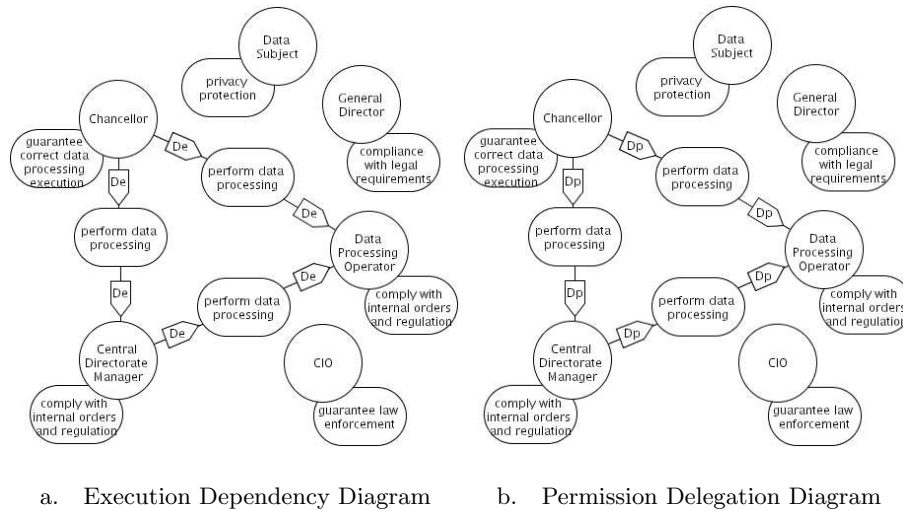
Figure 8. Requirements Model
