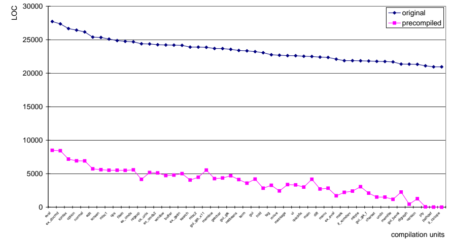
Size of preprocessed compilation units in LOC (VIM 6.2)
