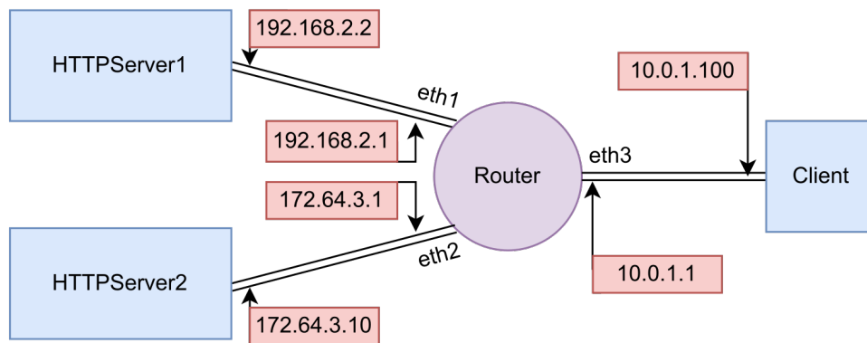
Figure 1: Sample routing topology
