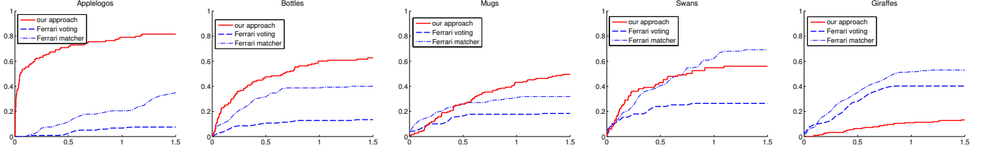
Figure 6. Comparison with Ferrari et al. , training without bounding boxes.
