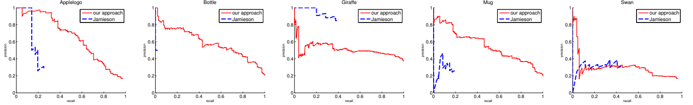
Figure 5. Comparison with Jamieson et al. Contour features capture object categories more effectively than appearance-based features.
