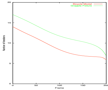
Figure 5: Number of iterations per frame (Bezier interpolation) decreases due to the addition of line constraints.
