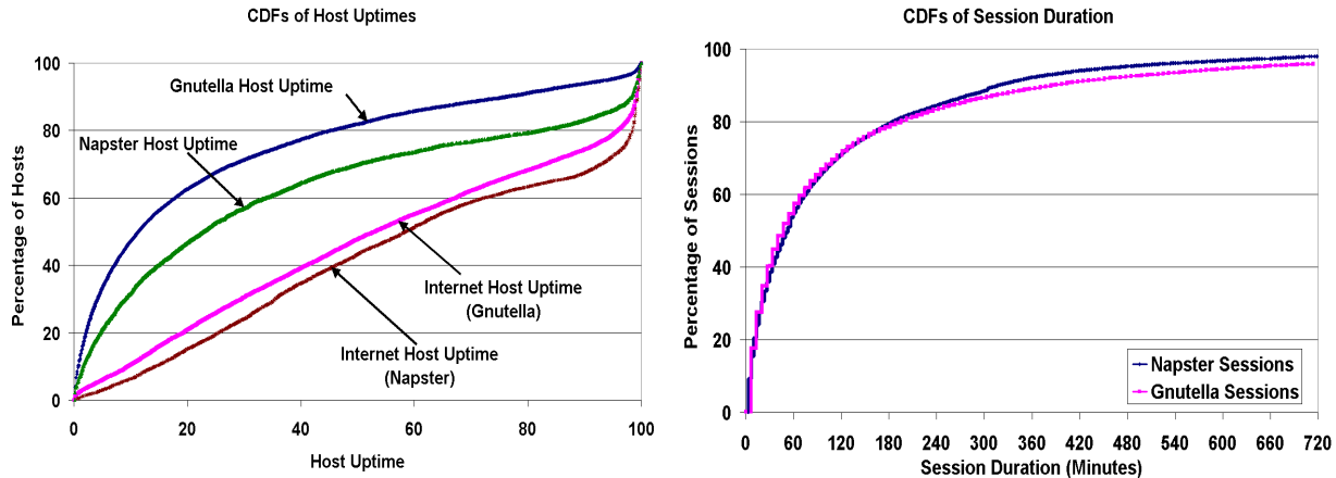
Figure 6. Left: IP-level uptime of peers (“Internet Host Uptime”), and application-level uptime of peers (“Gnutella/Napster Host Uptime”) in both Napster and Gnutella, as measured by the percentage of time the peers are reachable; Right: The distribution of Napster/Gnutella session durations.
