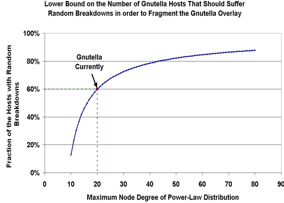
Figure 12. Lower bound on the number of Gnutella peers that must suffer random breakdowns in order to fragment the Gnutella network.
