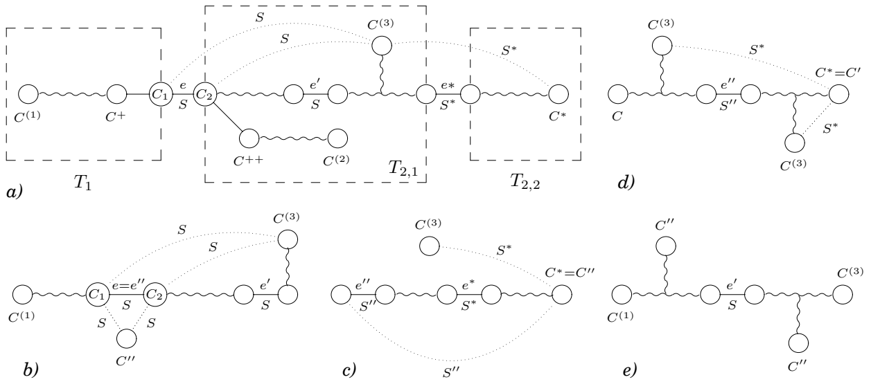
Figure 3: Cases in the proof of Theorem 14.
