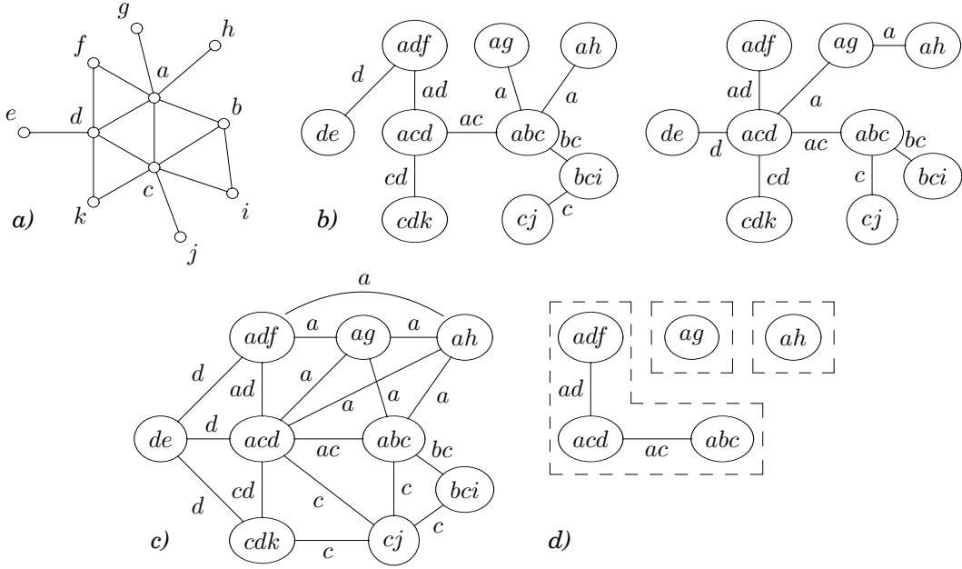
Figure 1: a) G , b) two example clique trees of G , c) C_r(G) , d) \mathcal{H}_{\{a\}}
