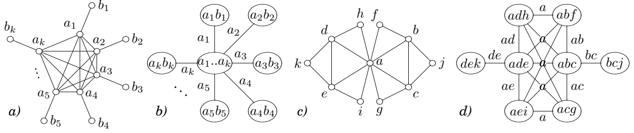
Figure 5: Examples of minimal forbidden split-minors.
