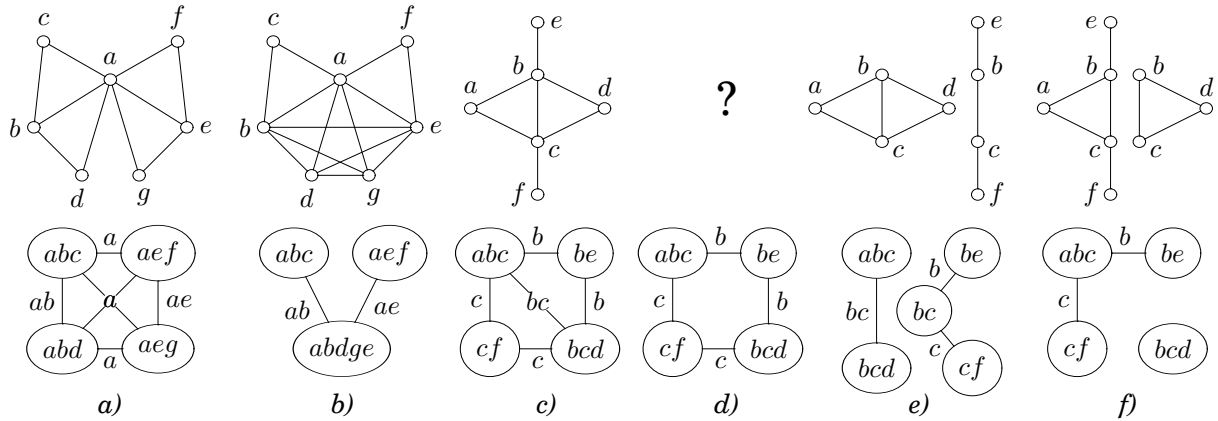
Figure 2: Examples justifying the definition of a split-minor.
