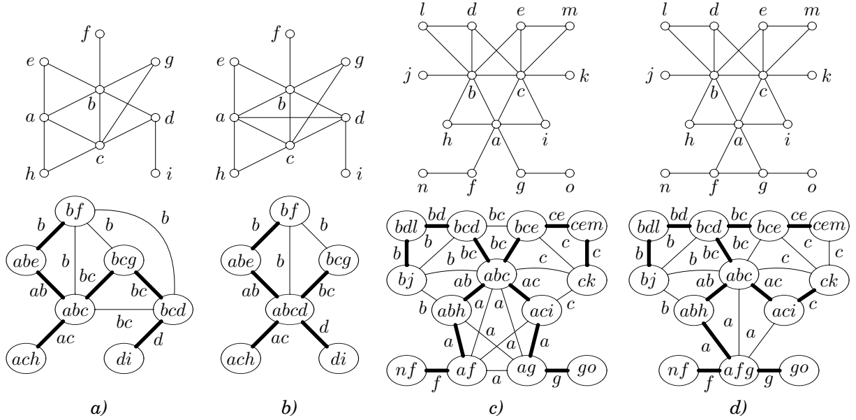
Figure 4: Examples justifying the definition of a good edge.
