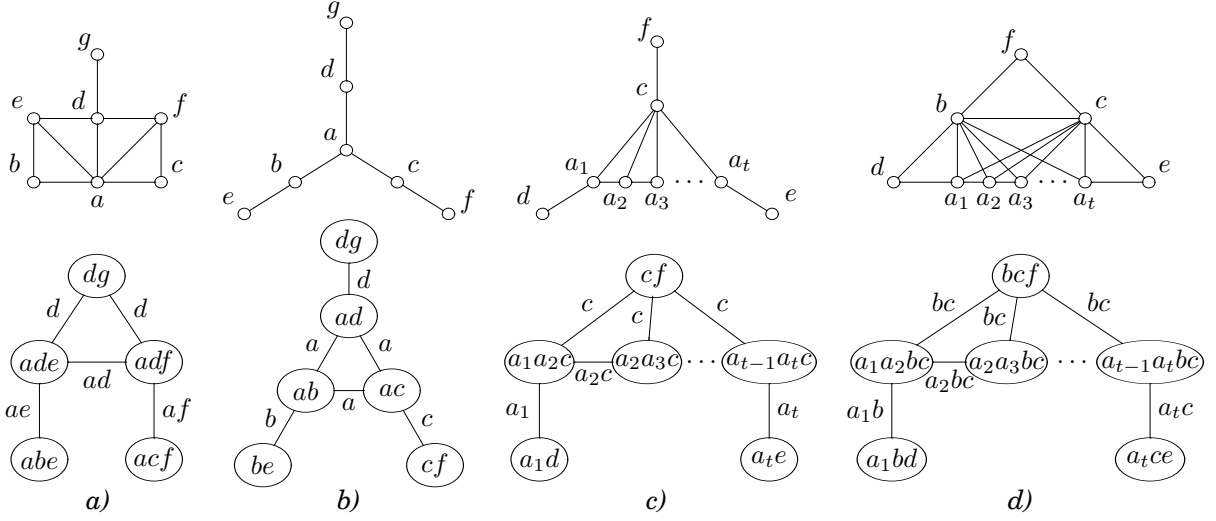
Figure 6: All chordal forbidden induced subgraphs for interval graphs and their reduced clique graphs (see [16]).
