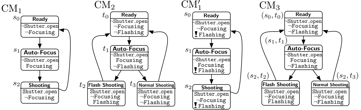
Figure 2. An example of merging state machines.
