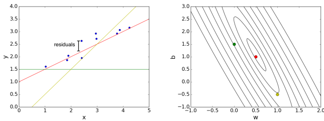
Figure 2: Contour plot of least-squares cost function for the regression problem.
