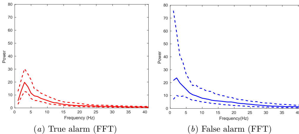
Figure 4: FFT of beats (lead II) - population median and IQR.
