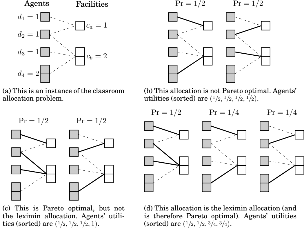
Fig. 1: Illustration of Example 3.1.
