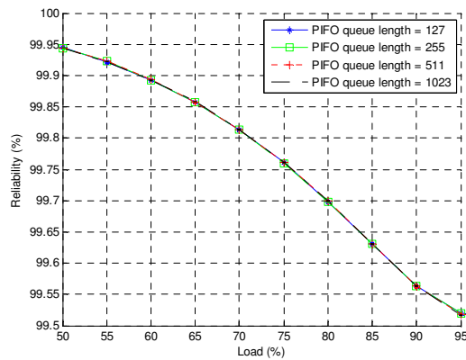
Fig. 5. Reliability of the optical PIFO buffer versus load.
