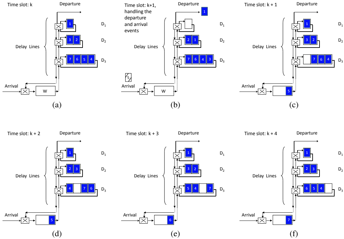
Fig. 3. Example of an emulated PIFO buffer.
