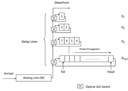
Fig. 1. Emulation of a FIFO buffer using fiber delay lines.
