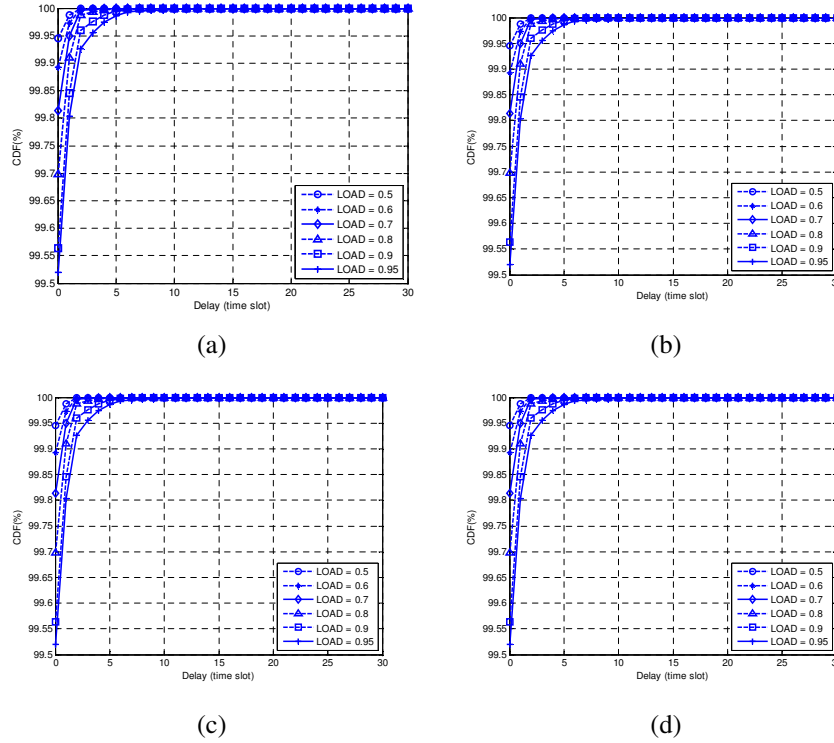
Fig. 6. Cumulative distribution function of departure delays (a) queue length = 127, (b) queue length = 255, (c) queue length = 511, (d) queue length = 1023.
