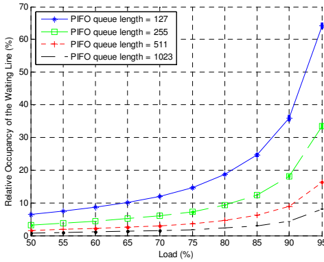
Fig. 7. Relative occupancy of the waiting line versus load.
