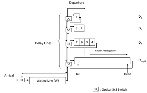
Fig. 2. Emulation of a PIFO buffer using fiber delay lines.
