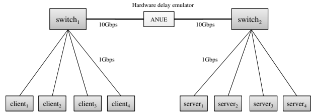
Fig. 1. Experiment's test-bed topology.
