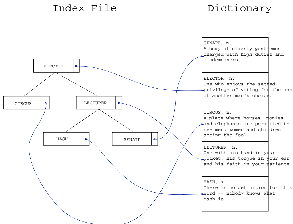
Figure 1: Logical structure of the Dictionary file and index file that might result from a number of calls to the add function.
