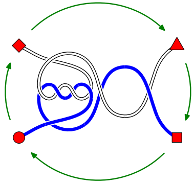
26: t = 10/7 - turn'em roun'
