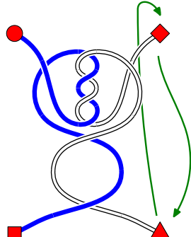
28: t = -7/10 - twist'em up
