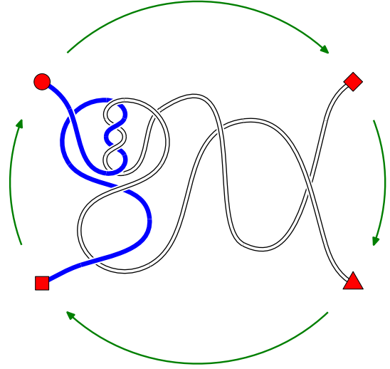
32: t = 13/10 - turn'em roun'
