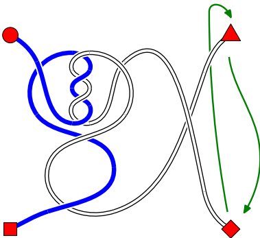
30: t = 3/10 - twist'em up
