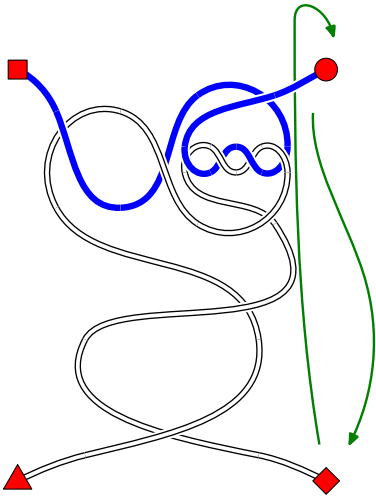
34: t = -10/13 - twist'em up
