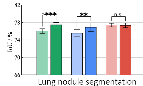
(c) Self-restoration
