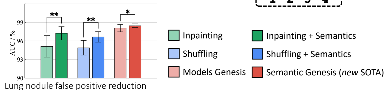
(b) Self-classification
