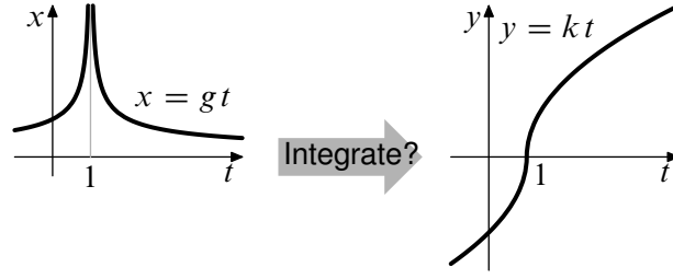
Figure 2: Integrand with a singularity.
