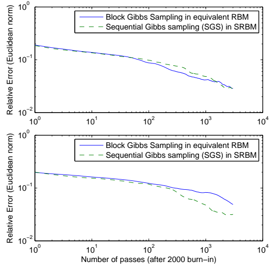
Figure 4: Relative estimation error (of the hx-statistic) versus step number for models trained on MNIST with the SRBM parameterization (bottom) and with the equivalent RBM parameterization (top).
