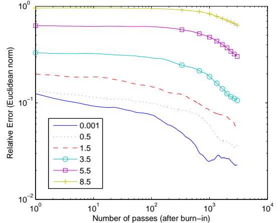
Figure 2: Error versus number of runs for the block-Gibbs chain running on the RBM constructed using \alpha = (1 + \epsilon)\alpha_{min} . The legend indicates the value of \epsilon used.
