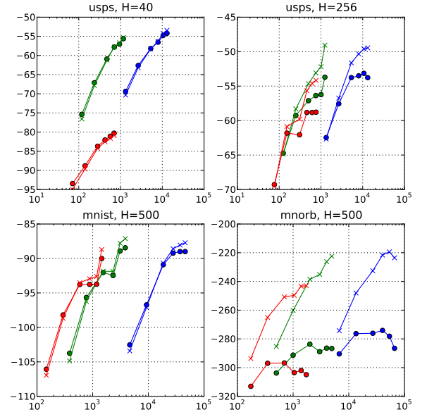
Figure 6: Plots showing the training and test log probabilities of the different models as learning progresses. Blue corresponds to the SRBM, green the equivalent RBM and red the standard 2-layer RBM without visible-visible connections. Circles correspond to the test set and x’s the training set. The x -axis is computation time in seconds, and the y -axis log probability.
