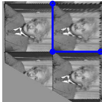
Similarity Reconstruction
