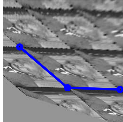
Affine Reconstruction
